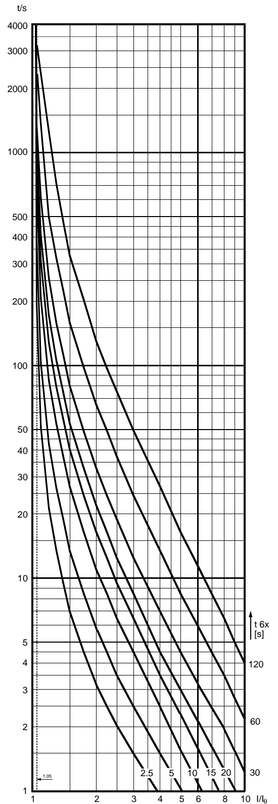
Fig. 2. Trip curves for the thermal unit with prior load 1.0 \times I_0 ("hot curve") at p = 100 \% .
